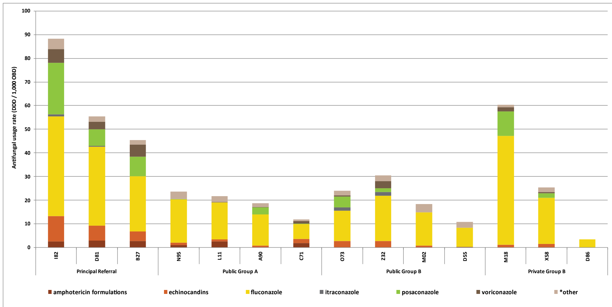
Chart 1: Total acute hospital antifungal usage rates (DDD/1000 OBD) in NAUSP contributor hospitals, by peer group, Western Australia, July-December 2023 (excluding emergency and theatre)
